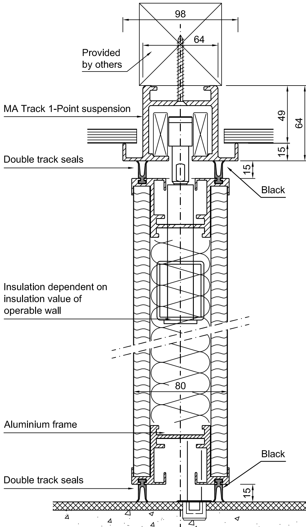
Section thru a typical type Multi Slide 85, Top hung
