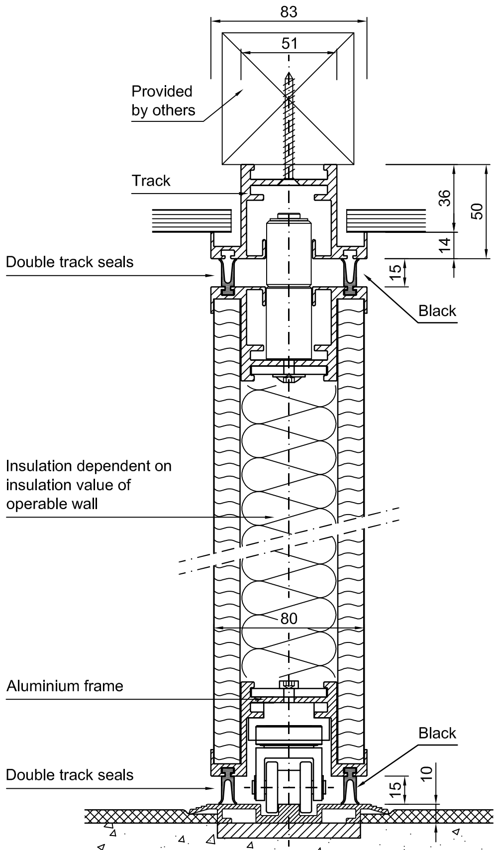
Section thru a typical type Multi Slide 85, Bottom Sliding
